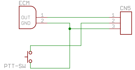
3-wire ECM and Push Switch
