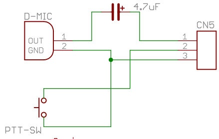
3-wire Dynamic MIC and Push Switch
