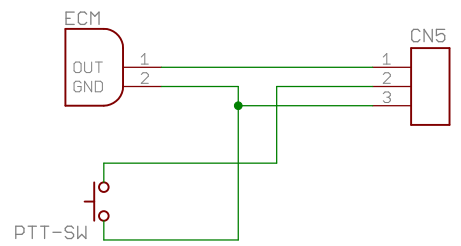
3-wire ECM and Push Switch
